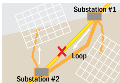
Scenario #2: Circuit Broken: Power re-routed through loop feed.
